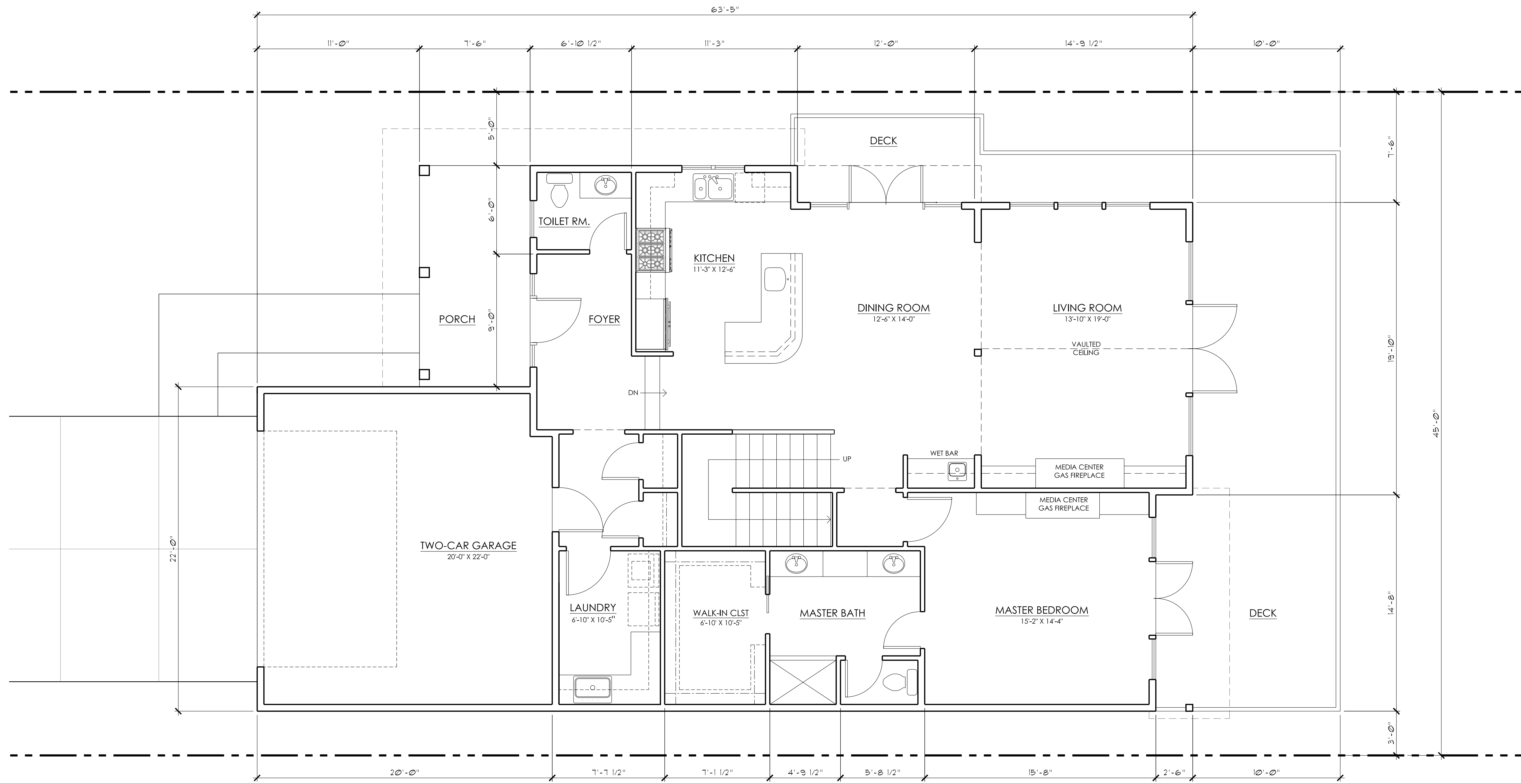
1 GROUND FLOOR PLAN HOUSE PLAN TYPE D A2.7 1/4" = 1'-0"
