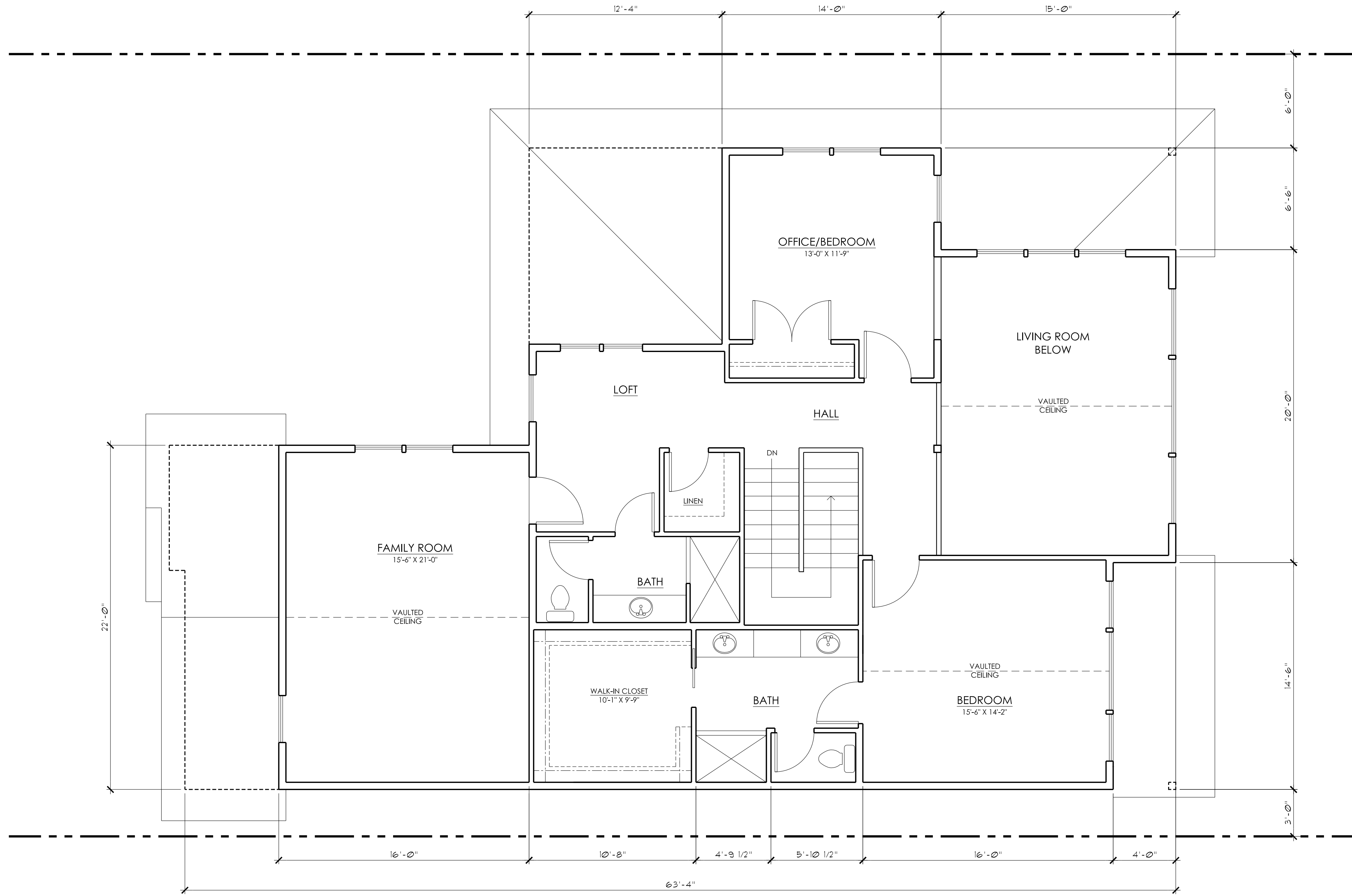
1 SECOND FLOOR PLAN HOUSE PLAN TYPE C A2.6 1/4" = 1'-0"
