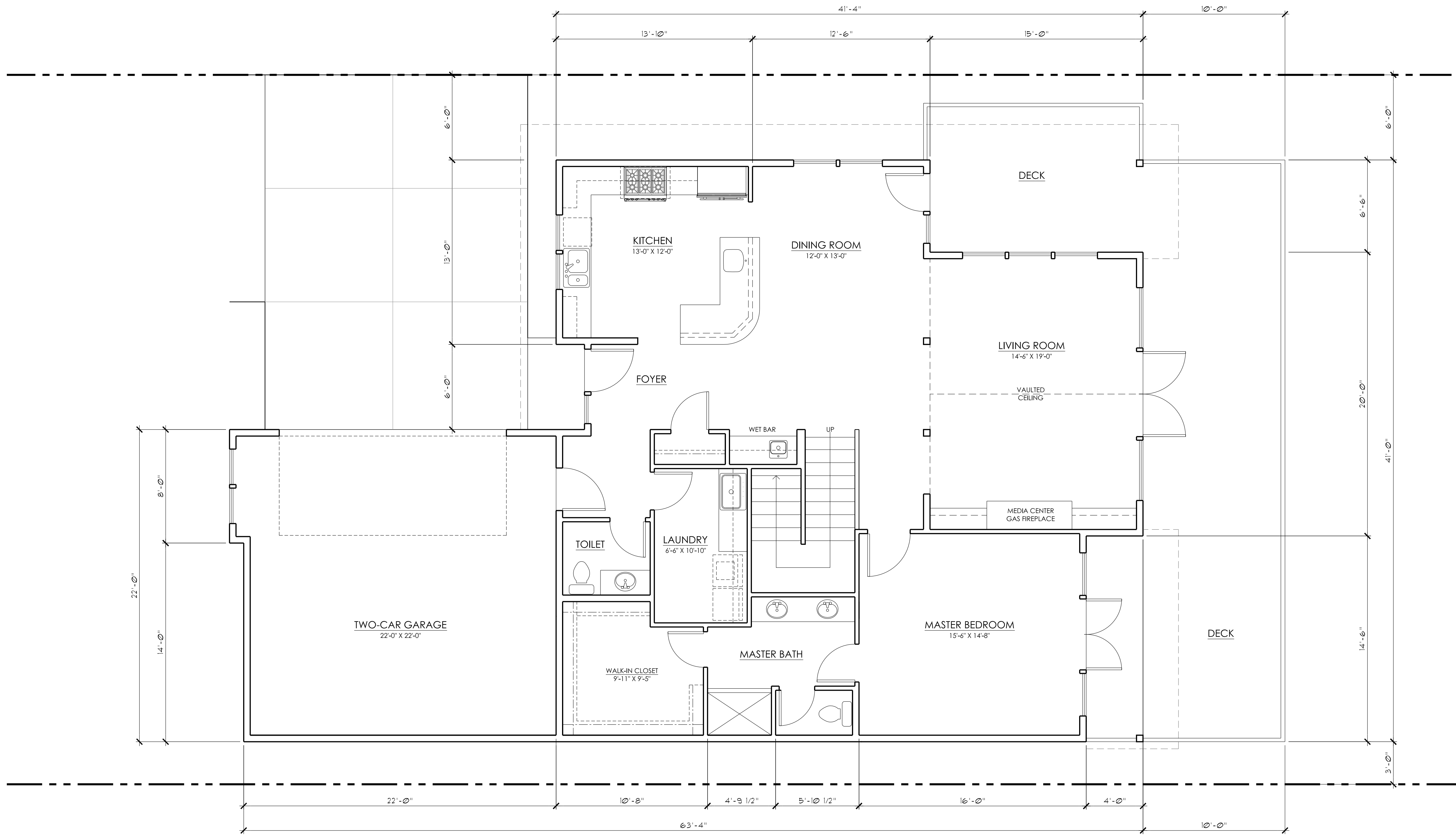
1 A2.5 GROUND FLOOR PLAN HOUSE PLAN TYPE C 1/4" = 1'-0"
