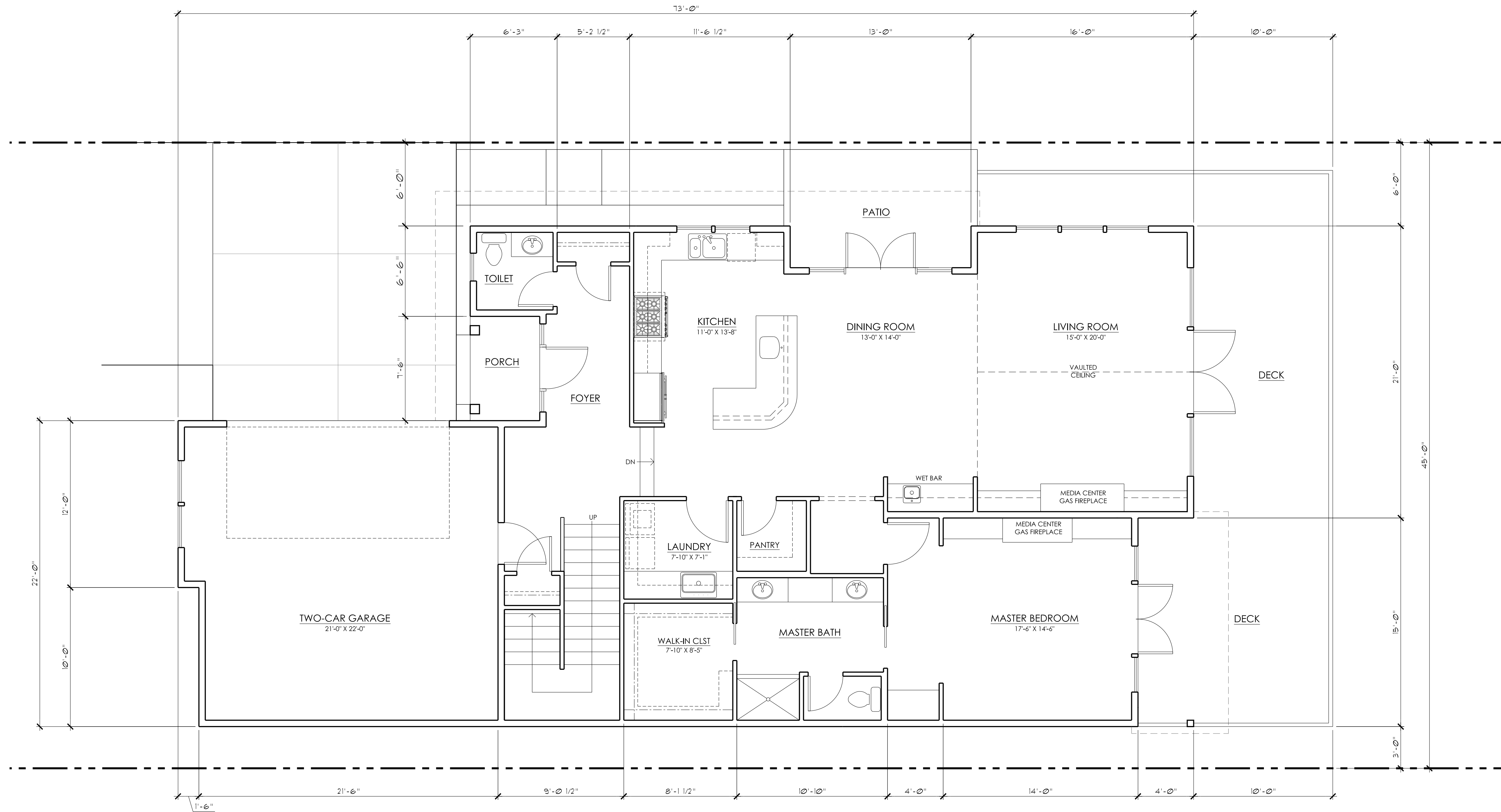
1 A2.3 GROUND FLOOR PLAN HOUSE PLAN TYPE B 1/4" = 1'-0"
